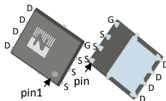
DFN5*6
